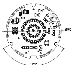
Fig1: RL-XMD070A series outline
