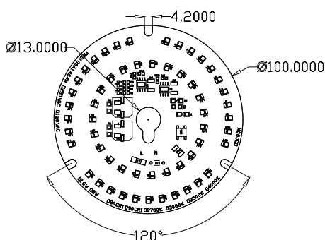
Fig2: RL-XMD100A series outline
