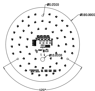
Fig3: RL-XMD180A series outline
