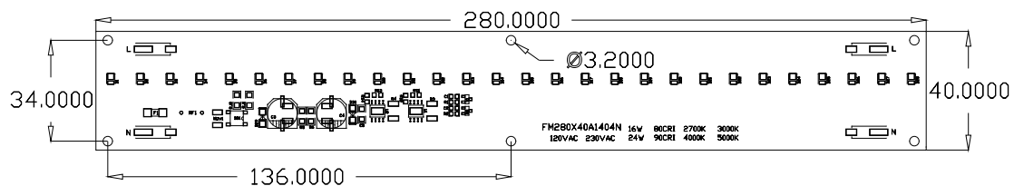
Fig1: RL-LM280*30Aseries outline
